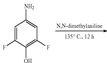
Compound (6)
