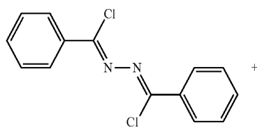
Compound (3)
