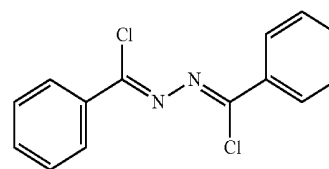
Compound (3)
