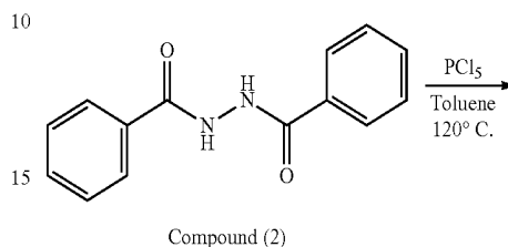
Compound (2)
