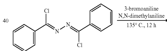
Compound (3)
