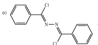
Compound (3)
