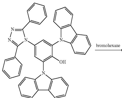
Compound (10)
