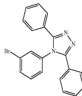
Compound (4)
