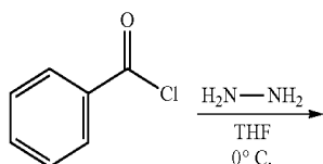
Compound (1)
