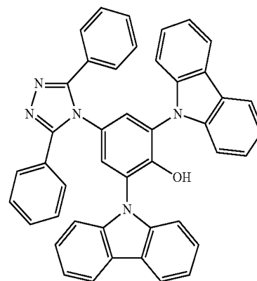
Compound (10)
