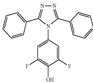
Compound (9)
