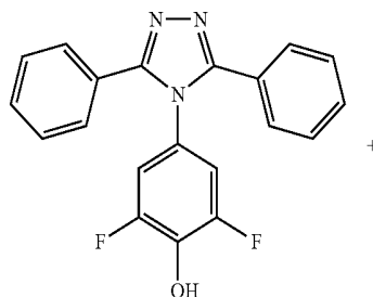
Compound (9)
