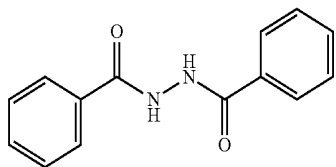
Compound (2)
